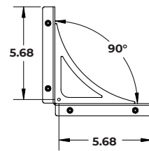
90° Bracket
