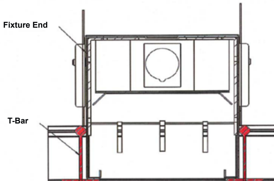
End View Detail C
