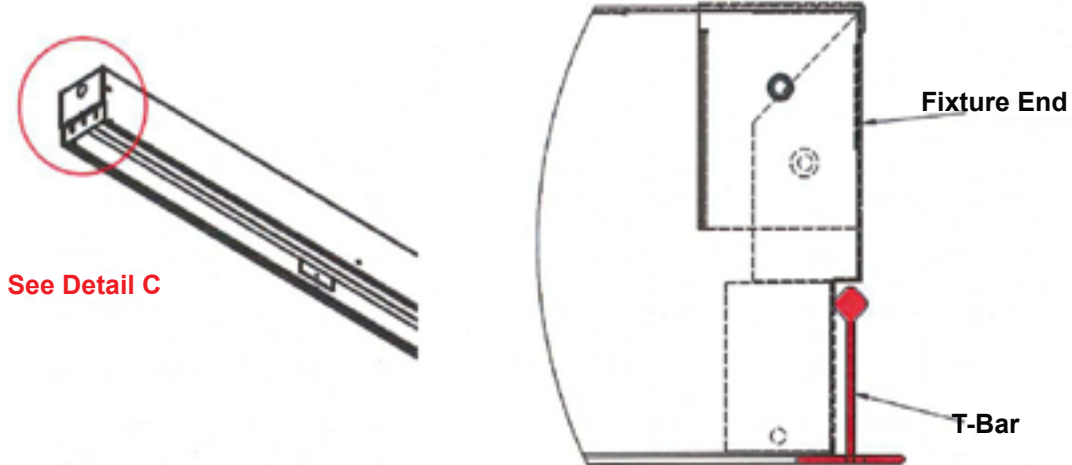
Side View Detail C
