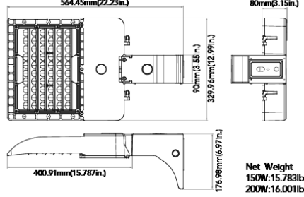
Pole Mount(150W&200W)
