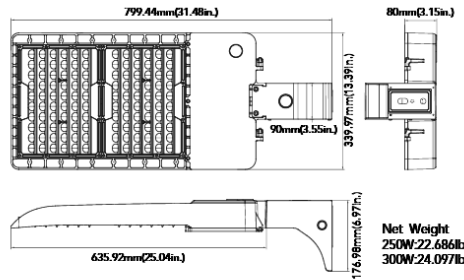
Pole Mount(250W&300W)
