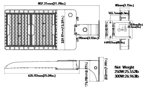
Wall Mount(250W&300W)
