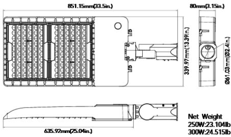
Slipfitter Mount(250W&300W)
