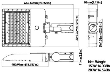
Slipfitter Mount(150W&200W)
