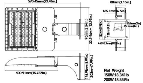
Wall Mount(150W&200W)
