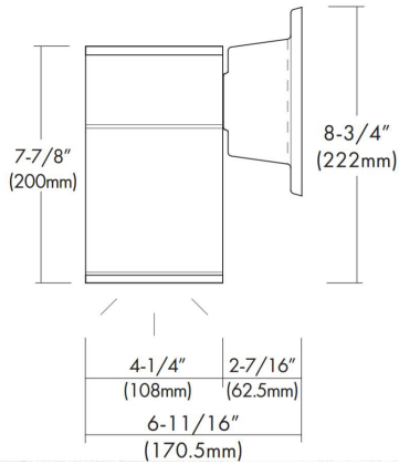
Wall Mount Downlight Only
