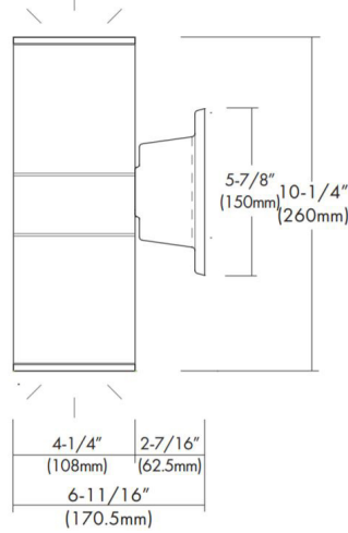
Wall Mount Up and Down Light
