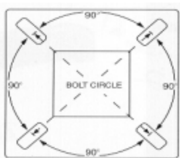
BOLT CIRCLE DIAGRAM FOR BOLT PLACEMENT
