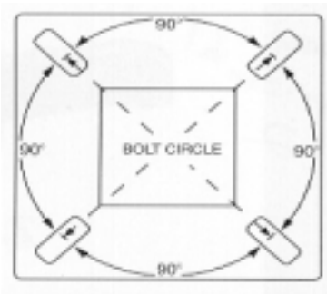
BOLT CIRCLE DIAGRAM FOR BOLT PLACEMENT
