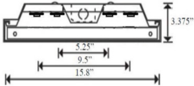
End Views
