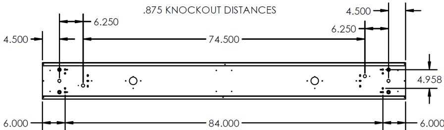
WIRE HANGING HOLE DISTANCES
