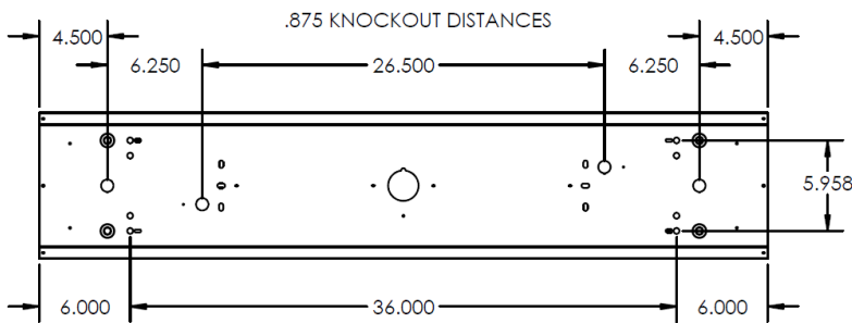
HANGING HOOK HOLE DISTANCES
